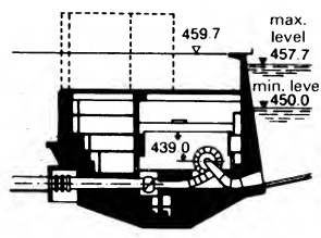
⑤ Power station with vertical Kaplan turbine (open air construction)
